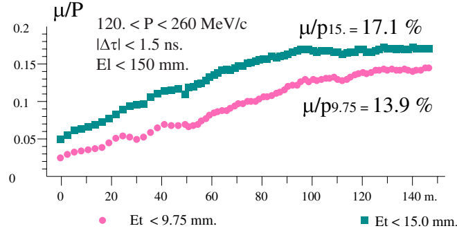
Figure 4.7: Geant4 simulations of the muon-to-proton yield ratio for two transverse emittance cuts, clearly showing that the channel cools, i.e. , the density in the center of the phase space region increases. Since the relevant yield \mu/p_{15} no longer increases for z \leq 110 m, the channel length was set to 108 m.
