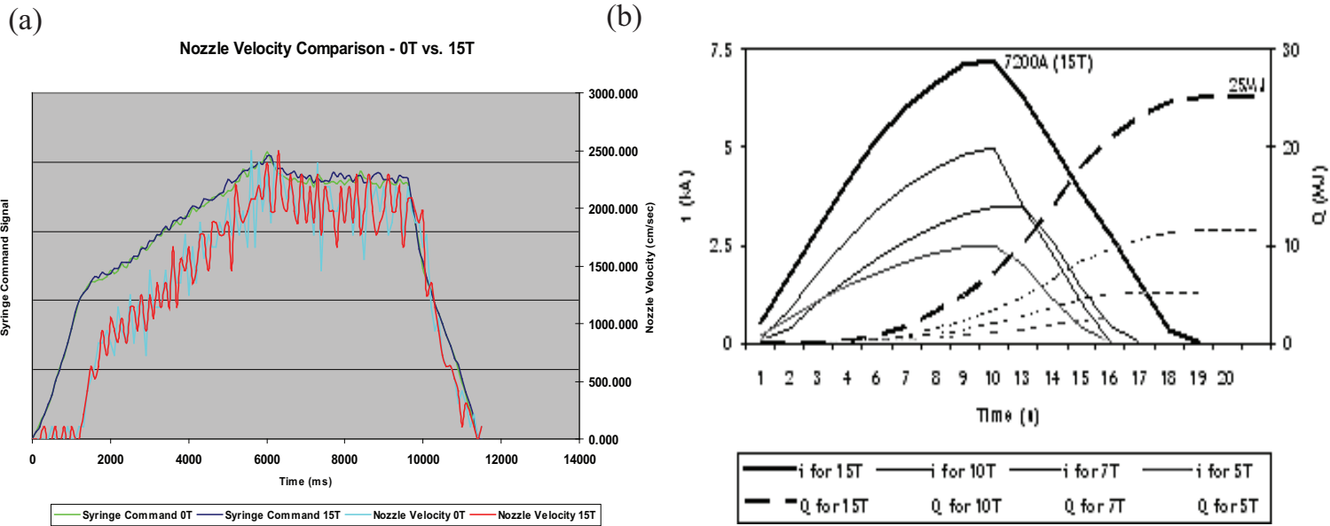
Figure 1.5: Operation of Hg loop system and pulsed 15 T solenoid magnet. a.) Hg loop system command [30]. b.) Behavior of the 15 T solenoid magnet during a pulse [42].
