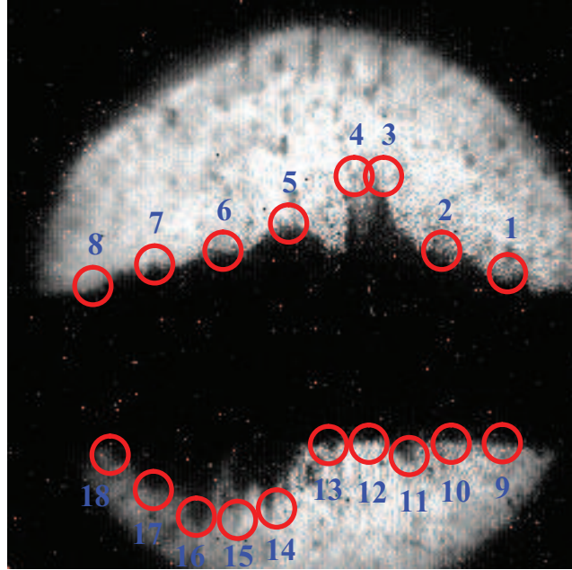
Figure 6.5: Location of 18 points of filament on the Hg jet surface for velocity measurement and its velocity. The shot condition is same with Fig. 6.3. The numbers above red circles point the filament that is used for velocity estimation in Fig. 6.6 and Fig. 6.7. a.) Location of filaments for measurement. b.) Filament velocity at each location.
