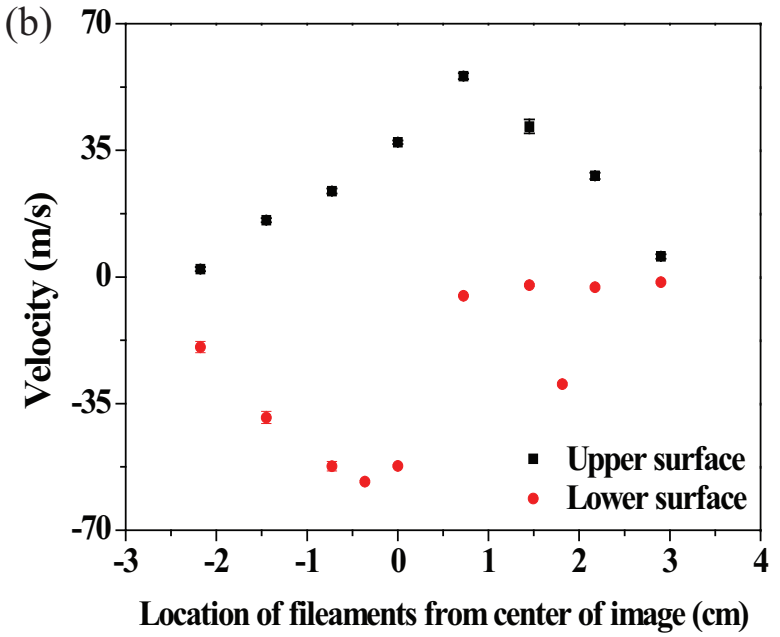
Figure 6.5: Location of 18 points of filament on the Hg jet surface for velocity measurement and its velocity. The shot condition is same with Fig. 6.3. The numbers above red circles point the filament that is used for velocity estimation in Fig. 6.6 and Fig. 6.7. a.) Location of filaments for measurement. b.) Filament velocity at each location.
