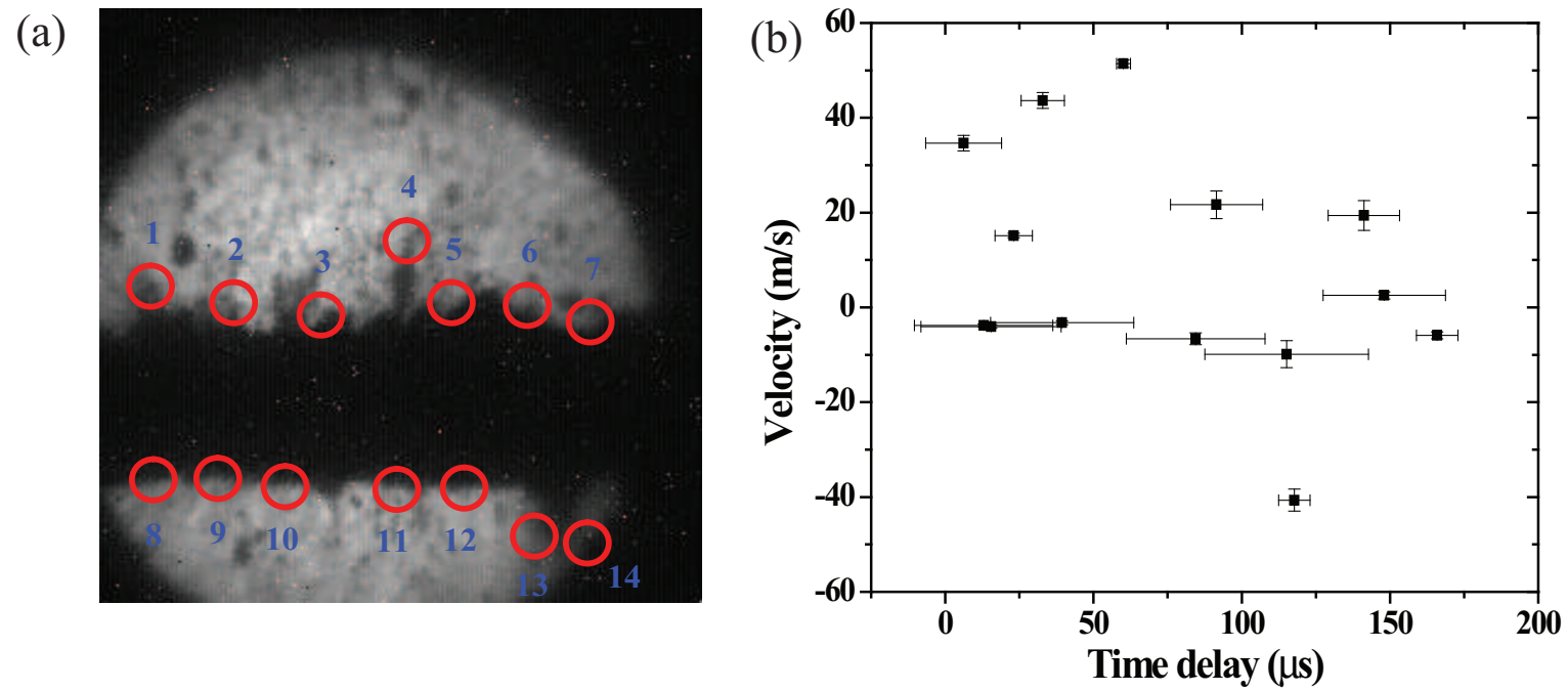
Figure B.12: Shot number is 12031. a.) Illustration of measured filaments. b.) Onset time of measured filament velocity.
