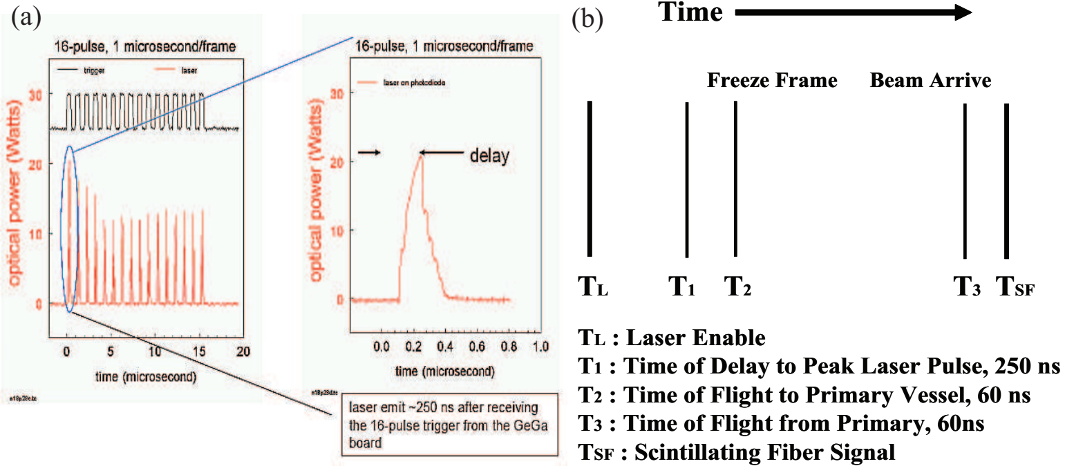
Figure 6.2: Time delay estimation of devices for triggered image calibration. a.) Measurement of characteristic response of 25 W laser used for high speed camera at Viewport 2 [92]. b.) Time structures between light source enabling and proton beam arrival.
