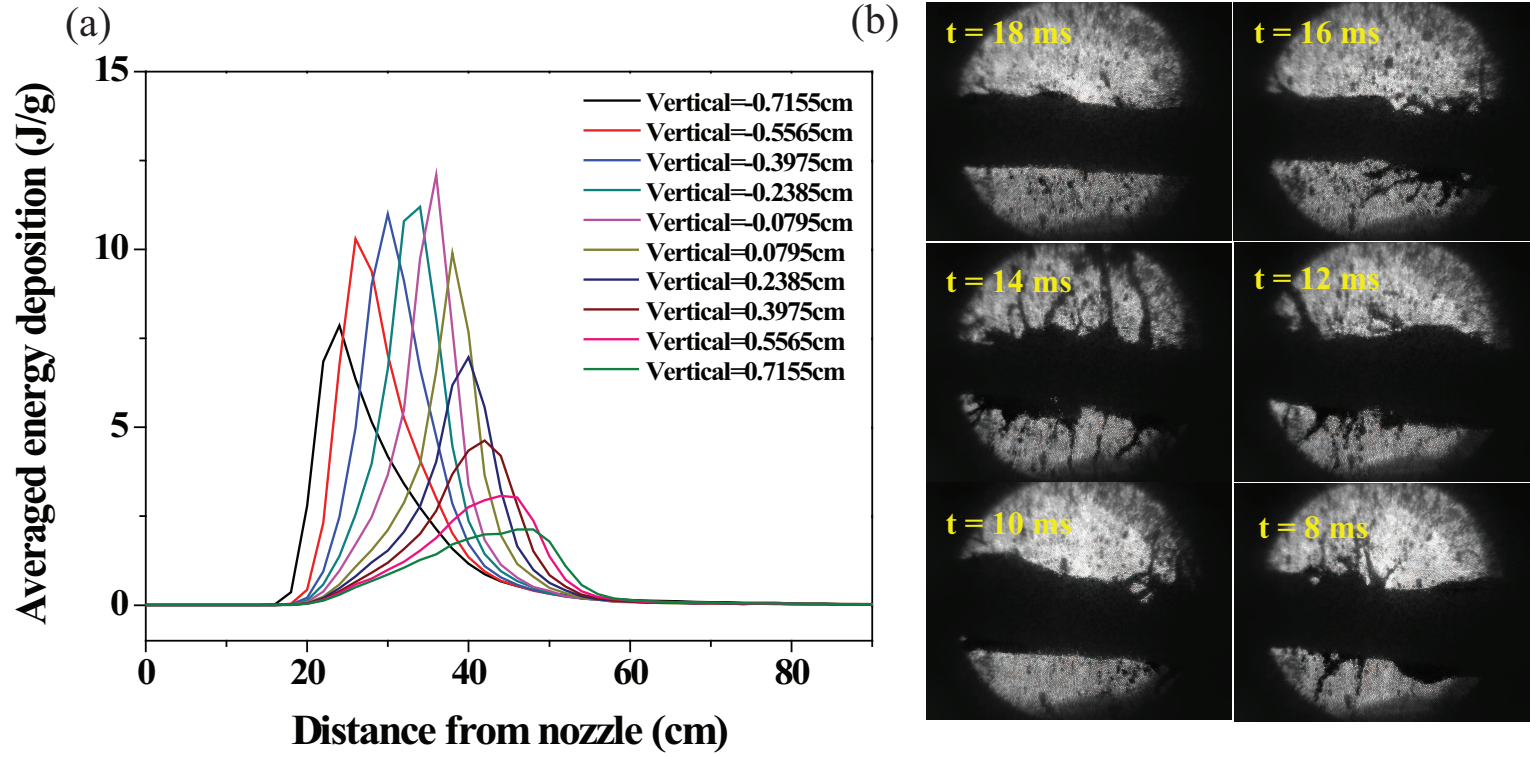
Figure 5.15: Qualitative comparison of the jet response by interaction of low intensity (3 Tp) of 24 GeV beam in 5 T. a.) Calculated averaged energy deposition using Eqn. (5.15) according to the vertical distance from jet center. b.) Observation of jet response by captured image.
