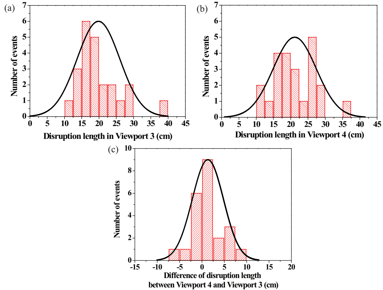
Figure 5.21: Validation of disruption measurement for the evaluation of evolution of disruption length from Viewport 3. a) Disruption length at Viewport 3. b.) Disruption length at Viewport 4. c.) Difference of the disruption length at Viewport 3 and Viewport 4.
