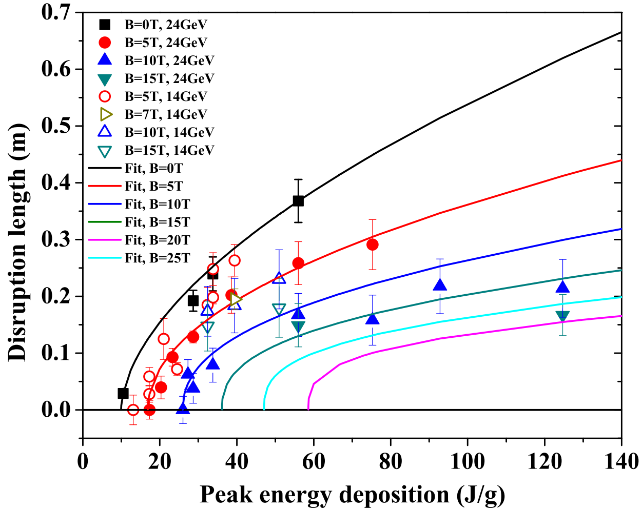
Figure 5.25: Disruption of mercury jet in magnetic fields as a function of peak energy deposition and fit of model using Eqn. (5.18).
