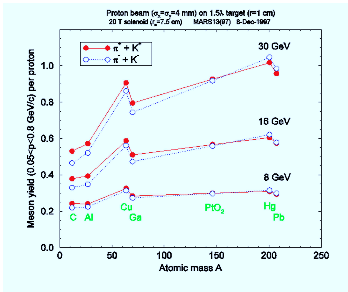
Figure 1.1: Pion yield versus atomic mass number of the target at three proton beam energies [66].
