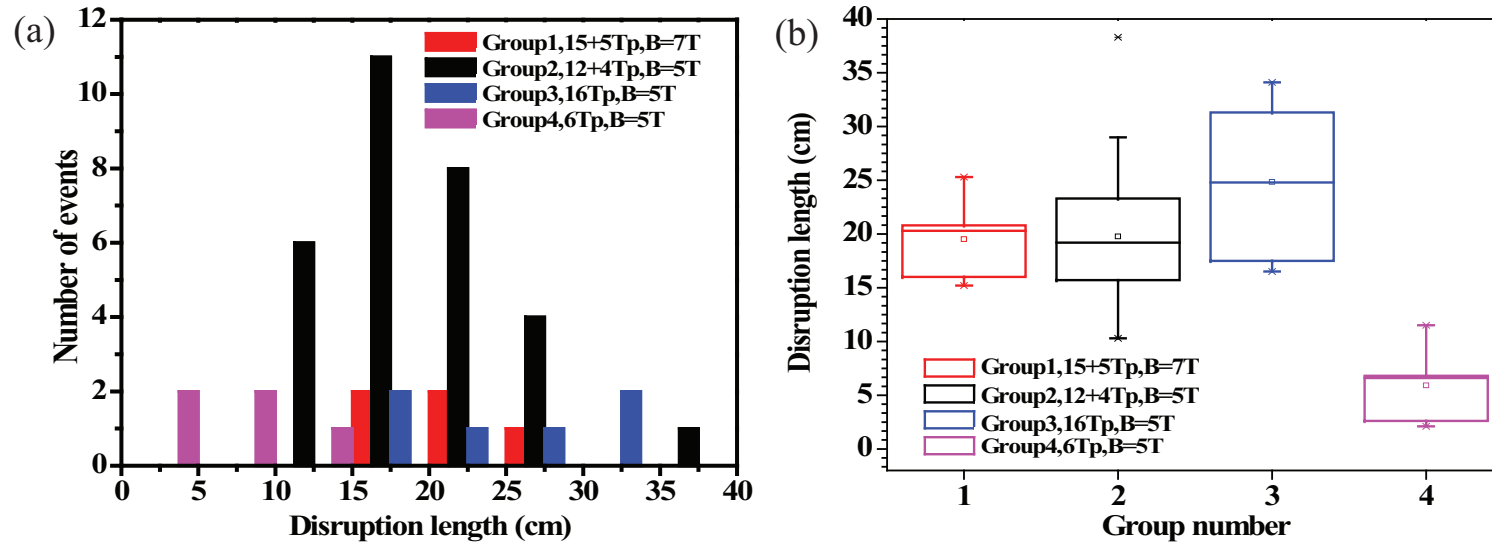
Figure 5.22: Disruption length measurement in same conditions. Pump-probe conditions with harmonic 8 and 16 bunches are used. The conditions of each group in pump-probe events are given in Table A.4. a.) Histogram of disruption length in each group. b.) Disruption length of each group.
