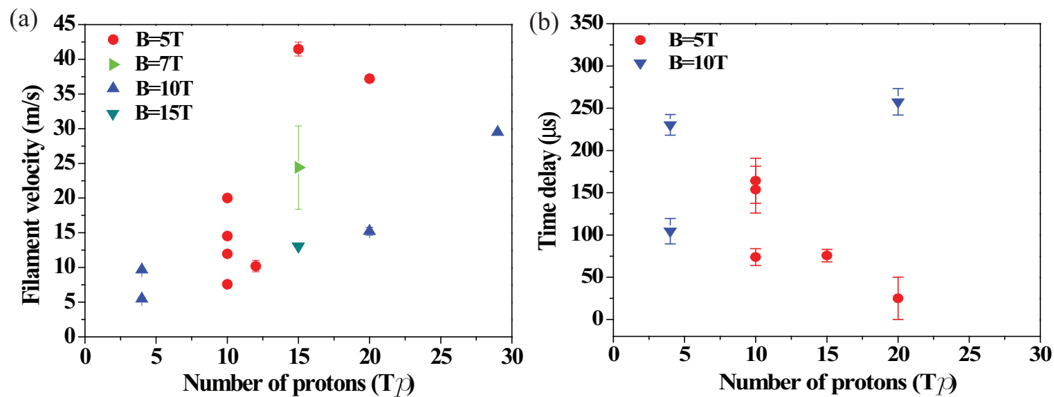
Figure 6.9: Maximum observed filament velocity as a function of 14 GeV beam intensity in various magnetic field. a.) Maximum observed filament velocity. b.) Onset time of that filament.
