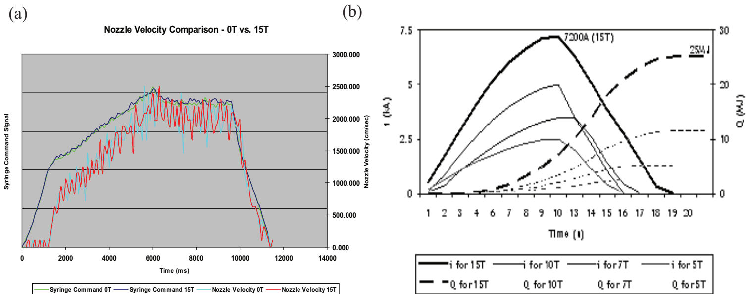
Figure 1.5: Operation of Hg loop system and pulsed 15 T solenoid magnet. a.) Hg loop system command [30]. b.) Calculated behavior of the 15 T magnet during a pulse [42].
