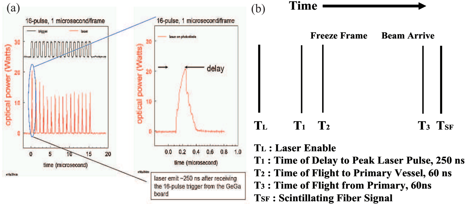
Figure 6.2: Time delay estimation of devices for triggered image calibration. a.) Measurement of characteristic response of 25 laser used for high speed camera at Viewport 2 [92]. b.) Time structures between light source enabling and proton beam arrival.
