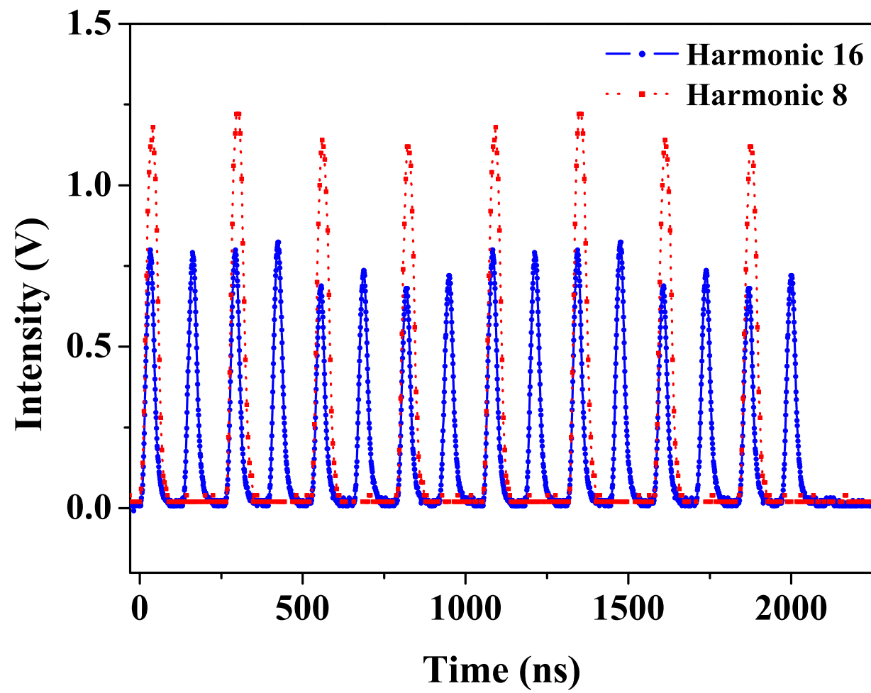
Figure 5.3: Proton beam pulse structure of harmonic 8 and harmonic 16 in 14 GeV and 6 Tp.
