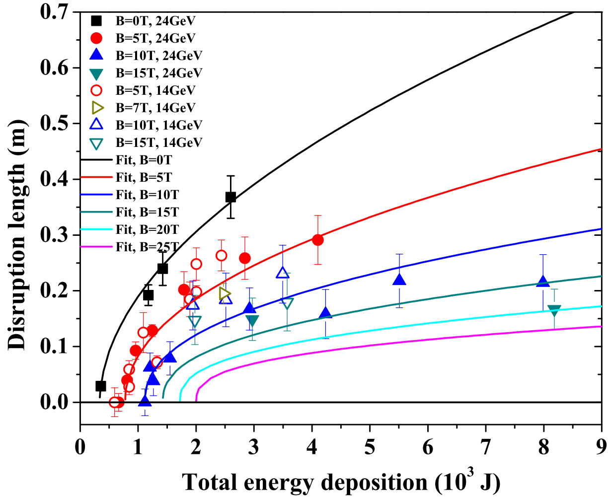
Figure 5.23: Disruption of mercury jet in magnetic fields as a function of total energy deposition and fit of model using Eqn. (5.18).
