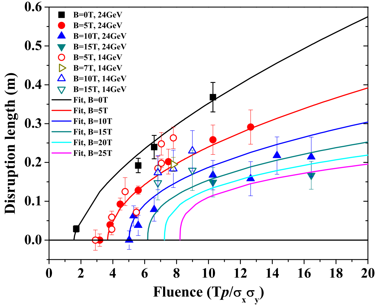
Figure 5.24: Disruption of mercury jet in magnetic fields as a function of fluence and fit of model using Eqn. (5.18).
