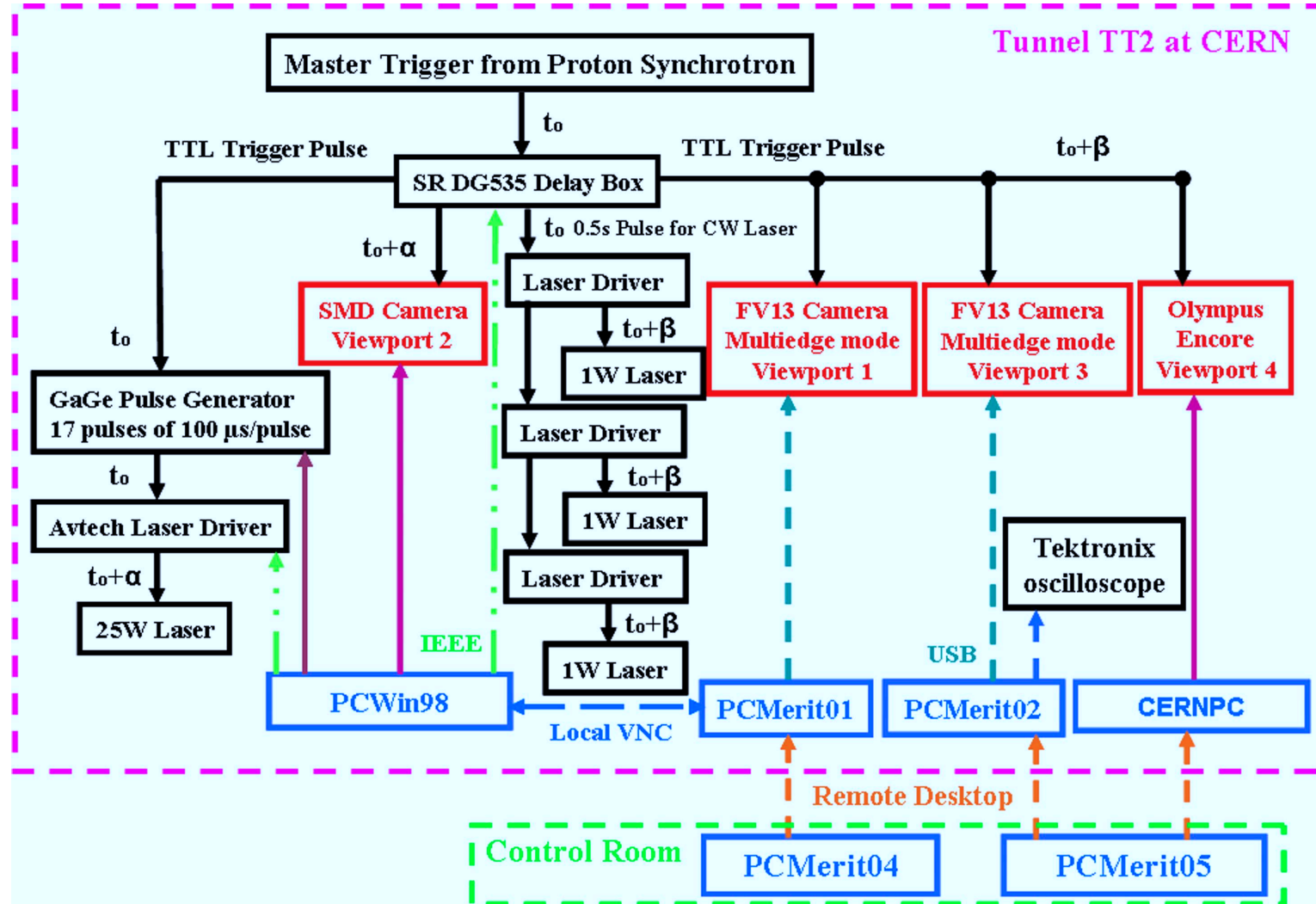
Figure 3.7: Schematic of electrical triggering and high speed camera control in tunnel for experiment.
