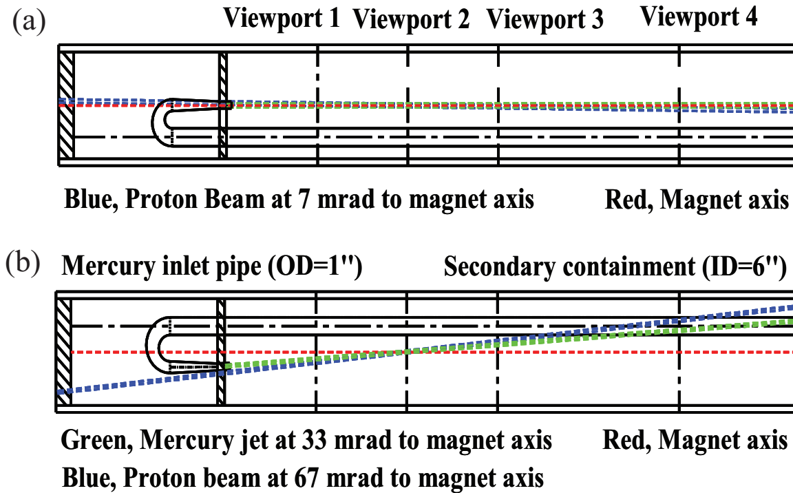
Figure 1.2: Geometry of key elements of target system and Viewports, showing the overlap between the mercury jet, magnetic axis, and the proton beam. a.) Top view. b.) Side view.
