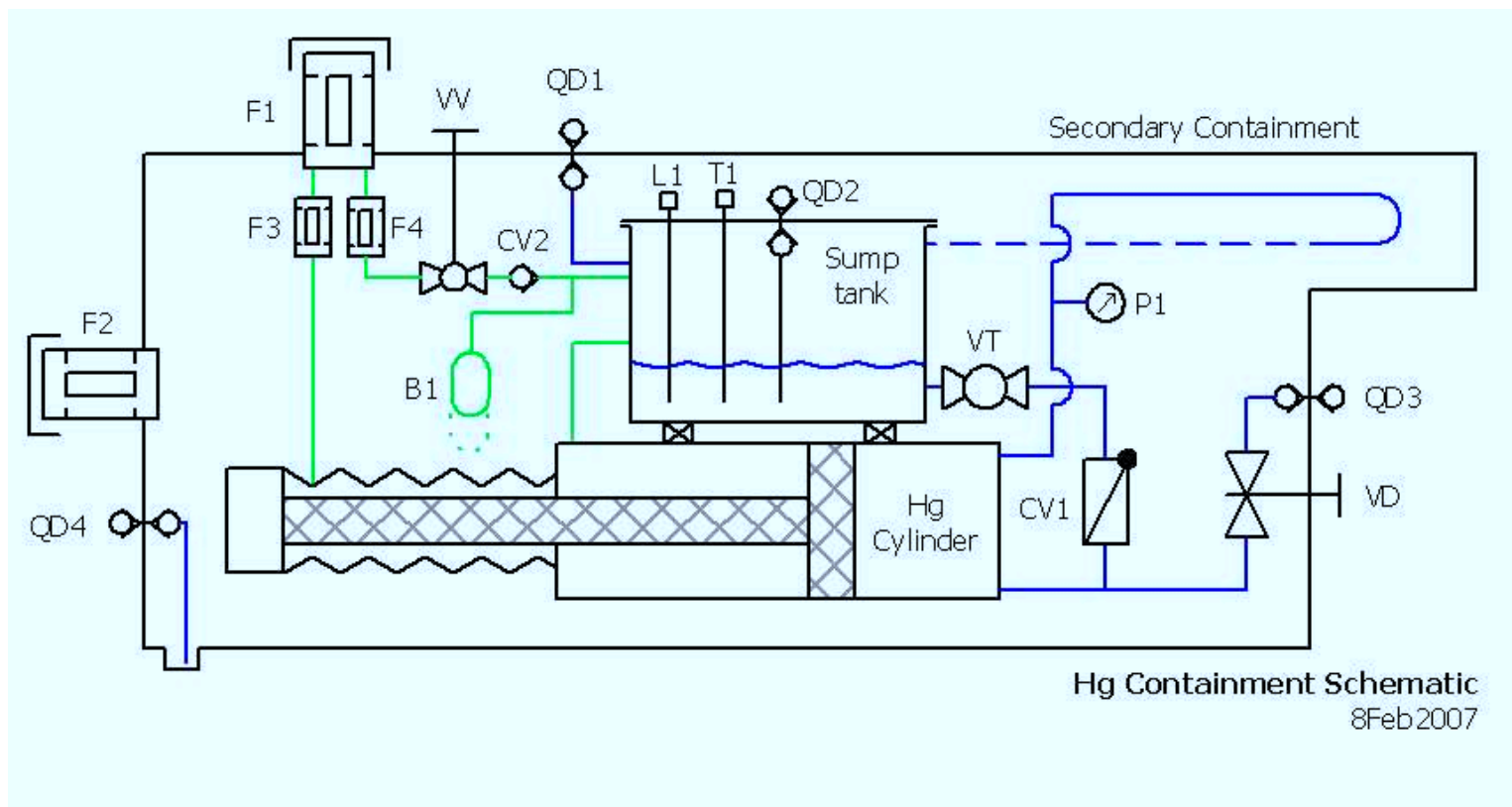
Figure 1.8: Schematics of mercury loop system for MERIT experiment [31].
