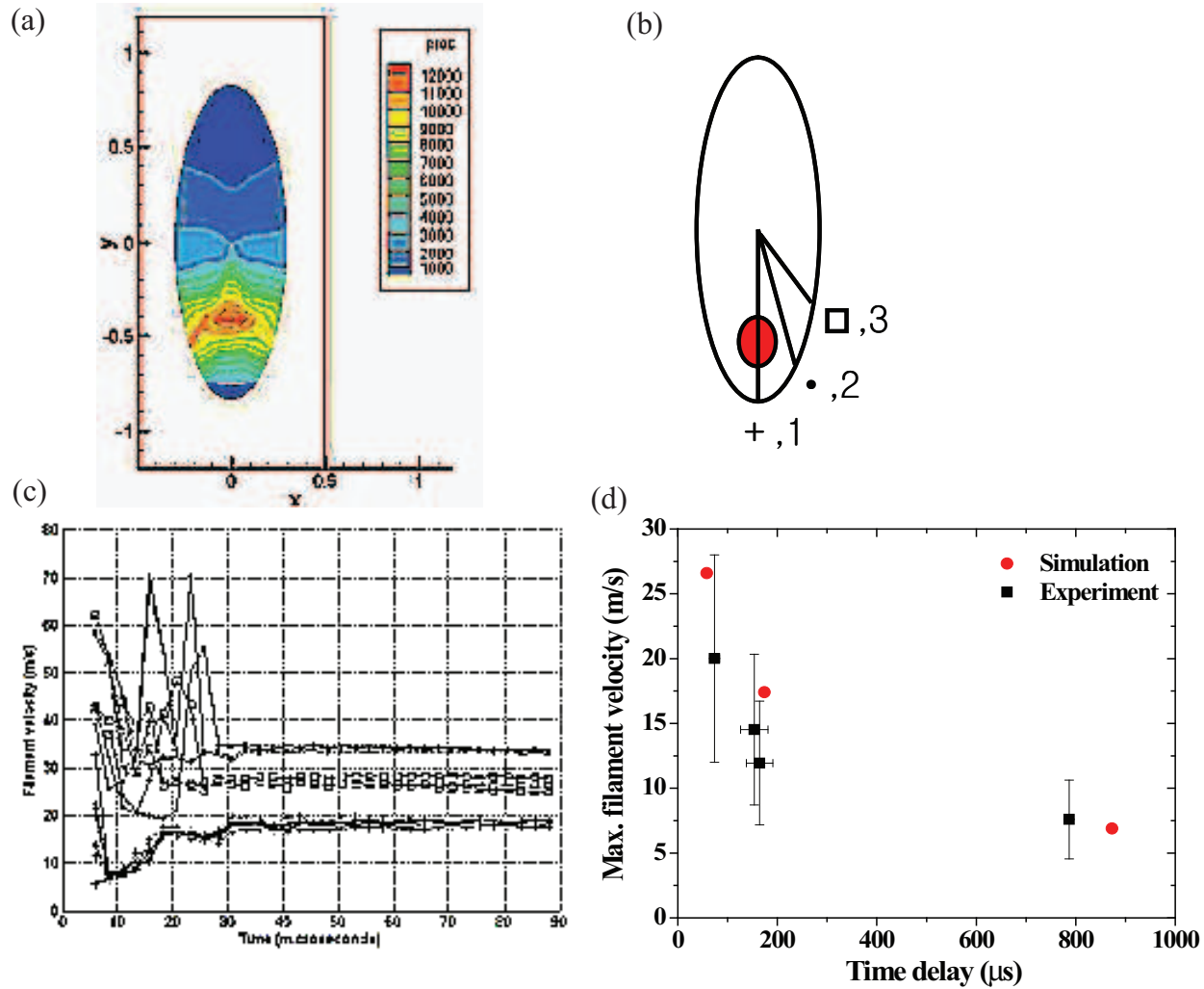
Figure 6.14: Comparison of calculated filament velocity with measurement. 14 GeV, 10 Tp and 0 T are considered in simulation. a.) Initial pressure contour in mercury jet by energy deposition [8]. b.) Location of picked filament for velocity calculation [7]. c.) Calculated filament velocity on the position 1, 2, and 3 [7]. d.) Apparent filament velocity in simulation and measurement.
