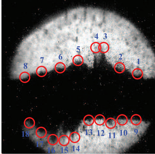
Figure 6.5: Filament velocity and location on the Hg jet surface for velocity measurement of 18 points of filament. The shot condition same with Fig. 6.3. The numbers above red circles points the filament that is used for velocity estimation in Fig. 6.6 and Fig. 6.7. a.) Location of filament for measurement. b.) Filament velocity at each location.
