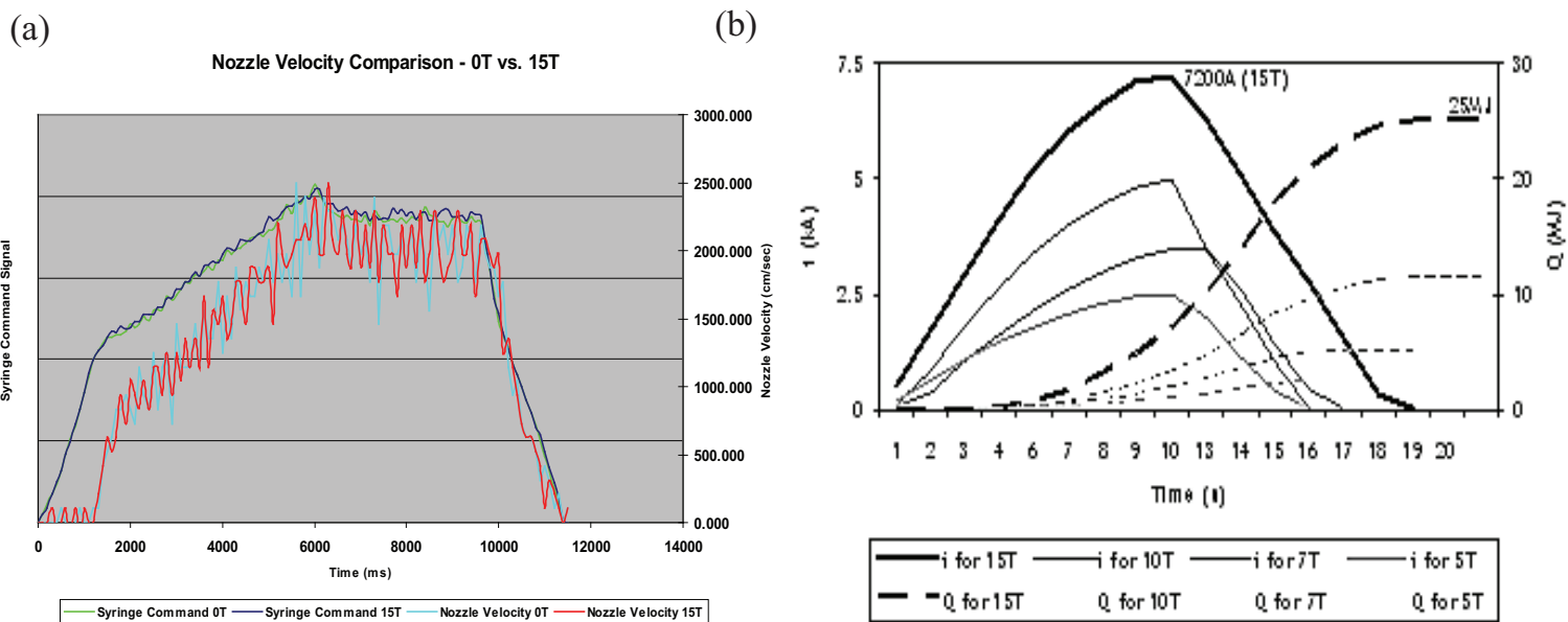
Figure 1.5: Operation of Hg loop system and pulsed 15 T solenoid magnet. a.) Hg loop system command [30]. b.) Calculated behavior of the 15 T magnet during a pulse [42].
