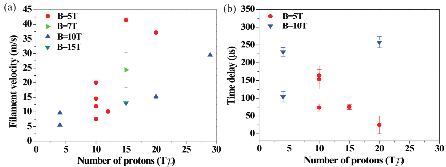
Figure 6.9: Maximum observed filament velocity as a function of 14\text{ GeV} beam intensity in various magnetic field. a.) Maximum observed filament velocity. b.) Onset time of that filament.
