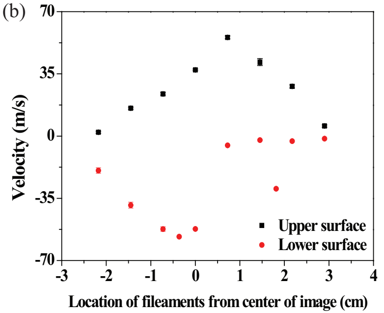
Figure 6.5: Filament velocity and location on the Hg jet surface for velocity measurement of 18 points of filament. The shot condition same with Fig. 6.3. The numbers above red circles points the filament that is used for velocity estimation in Fig. 6.6 and Fig. 6.7. a.) Location of filament for measurement. b.) Filament velocity at each location.
