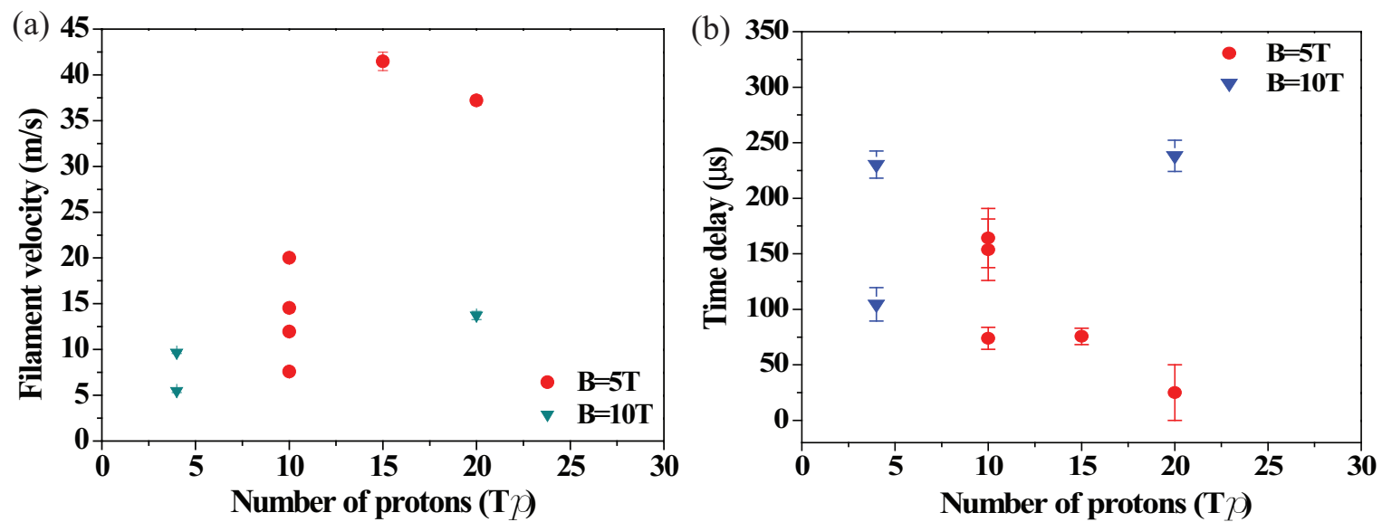
Figure 6.10: Filament velocity as a function of 14 GeV beam intensity and magnetic field. a.) Apparent filament velocity. b.) Onset time of filament.
