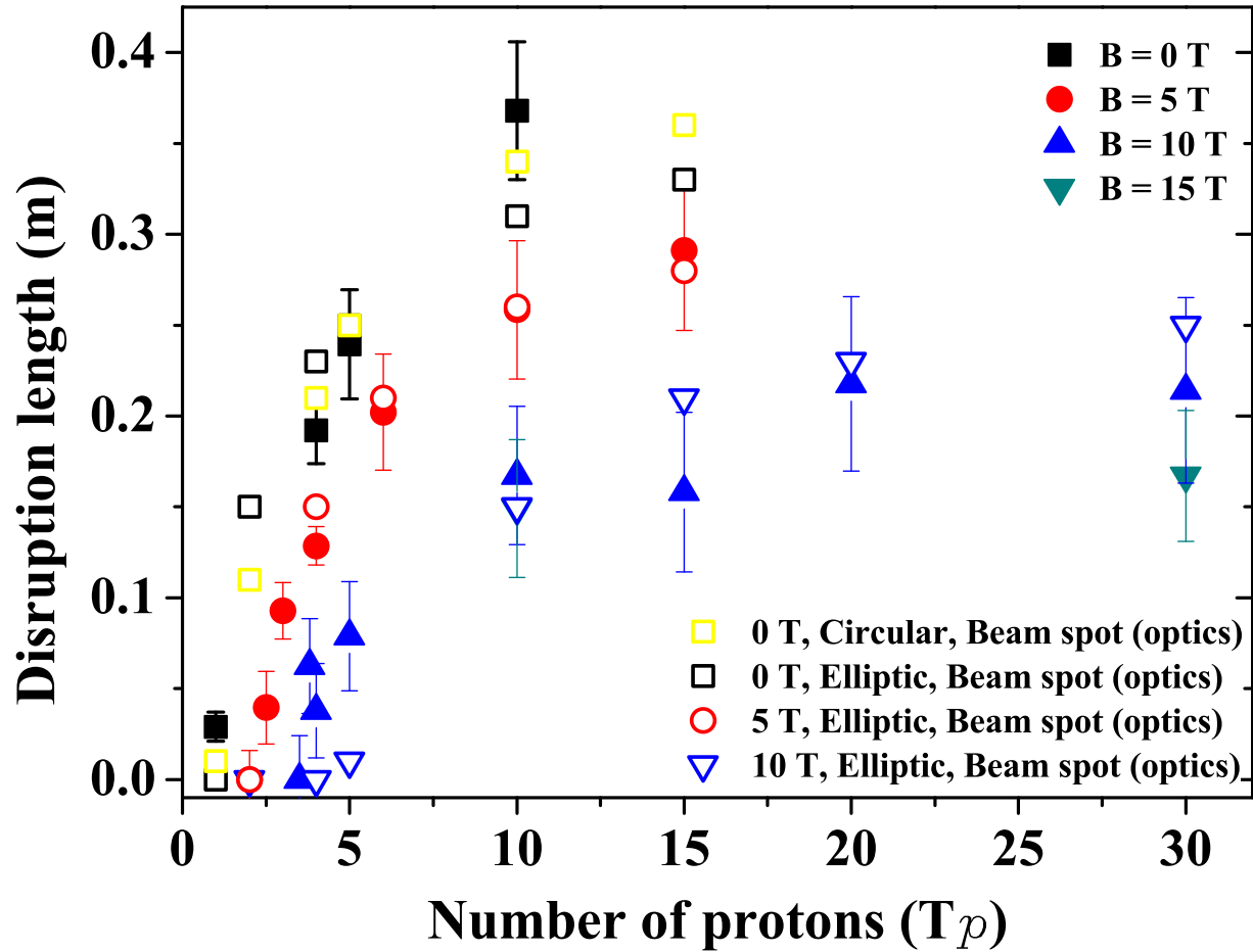
Figure 5.20: Disruption length of Hg jet and its estimation as a function of 24 GeV beam intensity and magnetic field.
