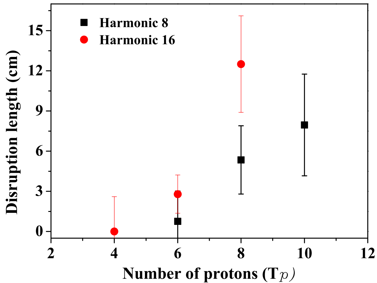
Figure 5.18: Disruption length of Hg jet depending on the beam pulse structure as a function of 14 GeV beam intensity in 5 T. T_p = 10^{12} protons.
