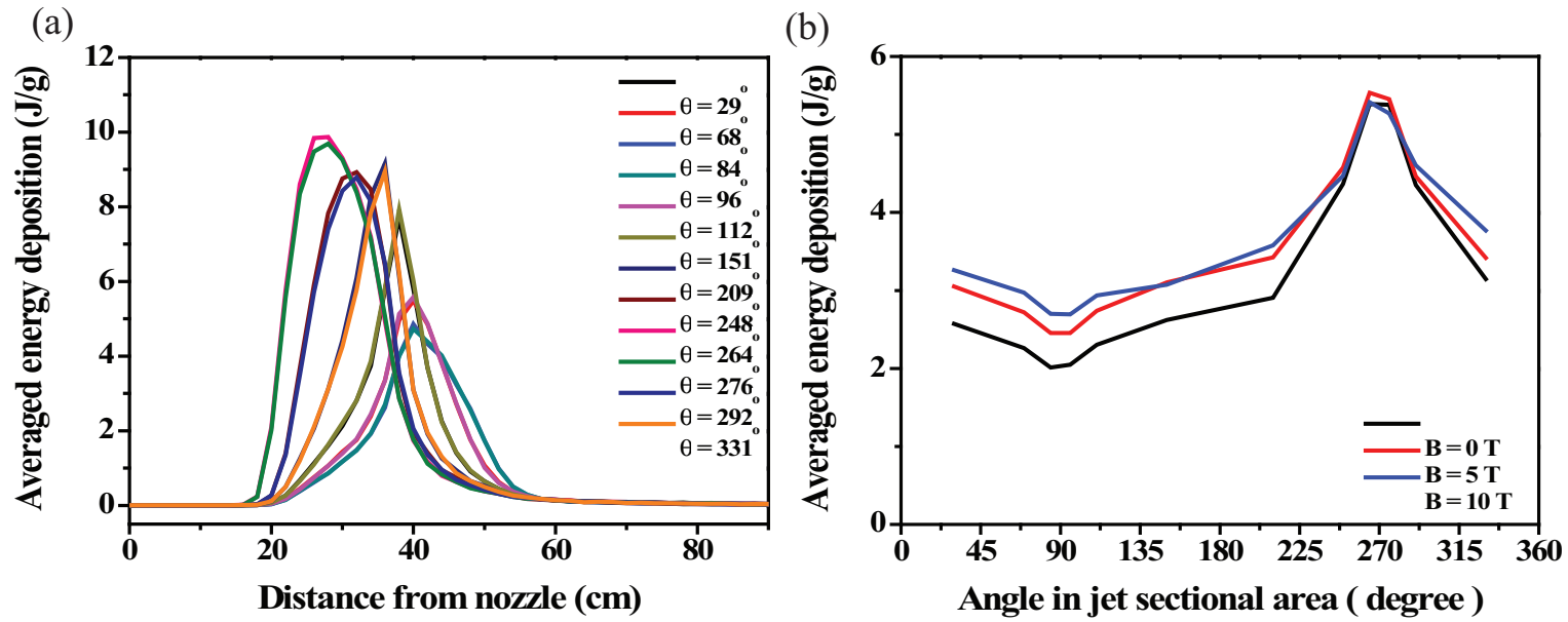
Figure 5.9: Radial energy deposition distribution along jet axis. a.) Along jet axis. b.) Along radial angle in jet cross section.
