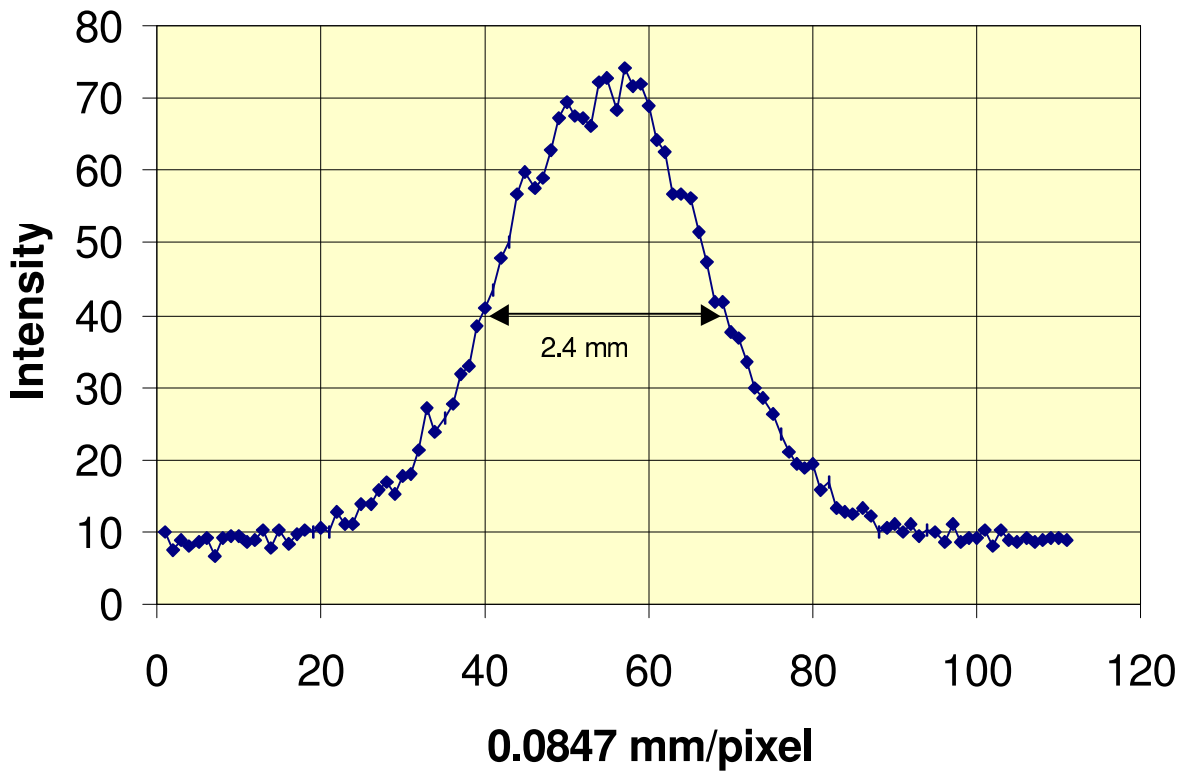
11 mils Havar - Horizontal Beam Profile
