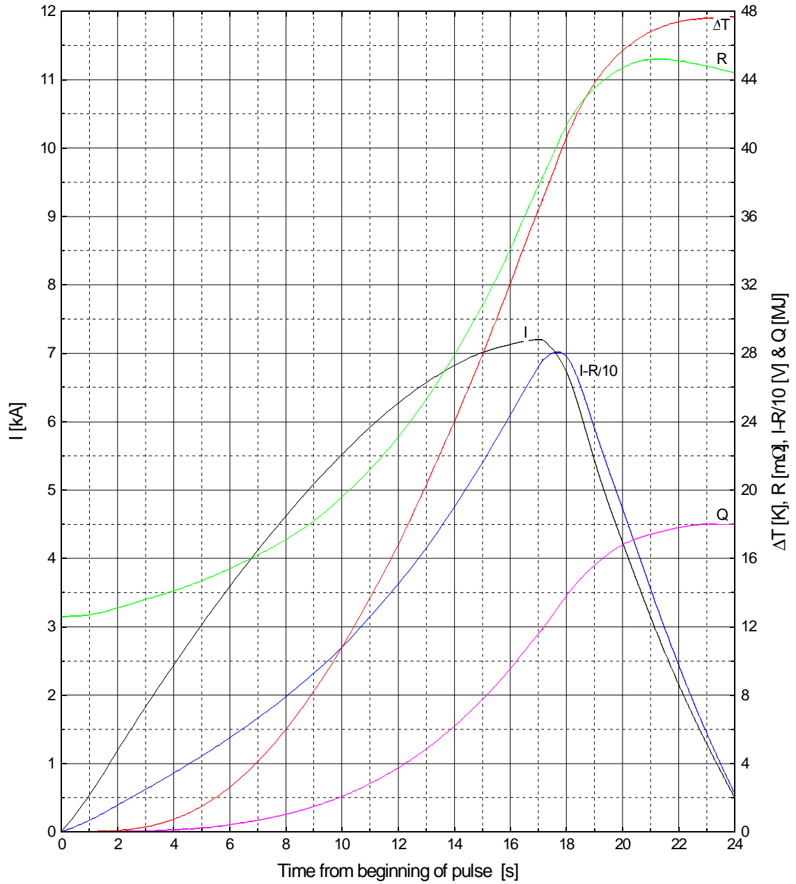
Current, Temperature Rise, Resistance, Resistive Voltage and Heating in E951 Magnet Precooled to 35.5 K and Pulsed at 300 Volts to 7.2 kA (14.5 T)
