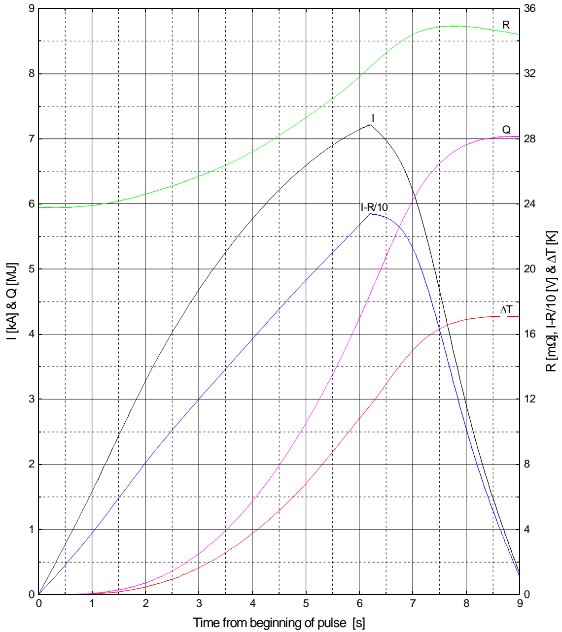
Current, Temperature Rise, Resistance, Resistive Voltage and Heating in E951 Magnet Precooled to 74 K and Pulsed at 300 Volts to 7.2 kA (10.1 T)
