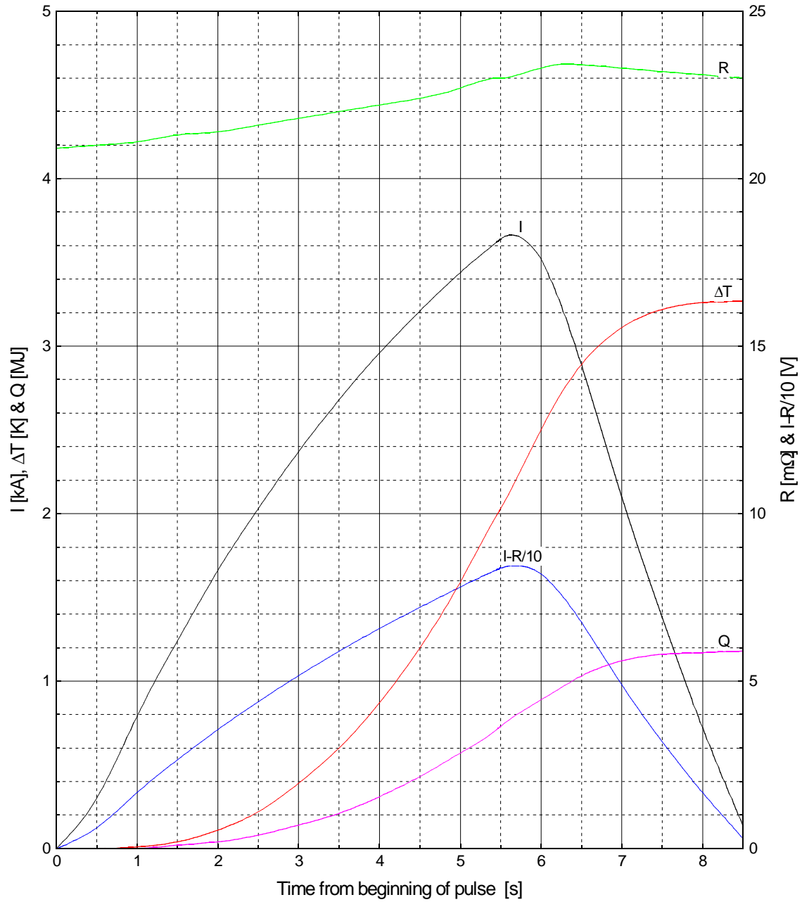
Current, Temperature Rise, Resistance, Resistive Voltage and Heating in E951 Magnet Precooled to 70 K and Pulsed at 150 Volts to 3.6 kA (5.0 T)
