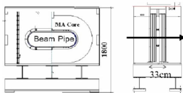
Fig. 22. 5 MHz ferrite-loaded cavity for FFAF scheme.
