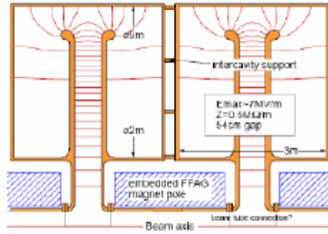
Fig. 21. 5 MHz vacuum cavity for FFAF scheme.
