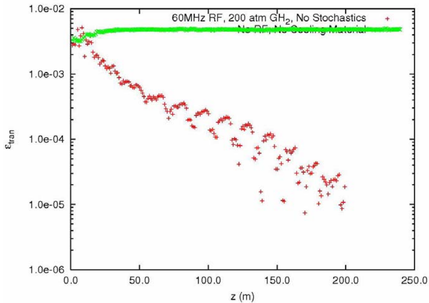
Transverse emittance
