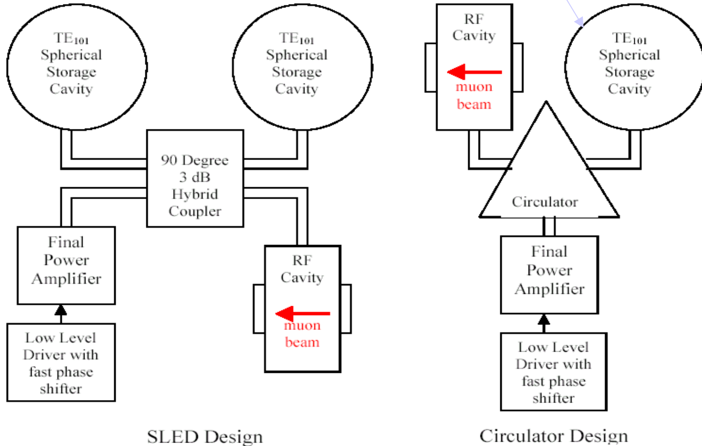
Figure 1. A comparison of the SLED and Circulator designs.
