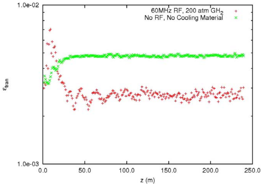
Transverse emittance
