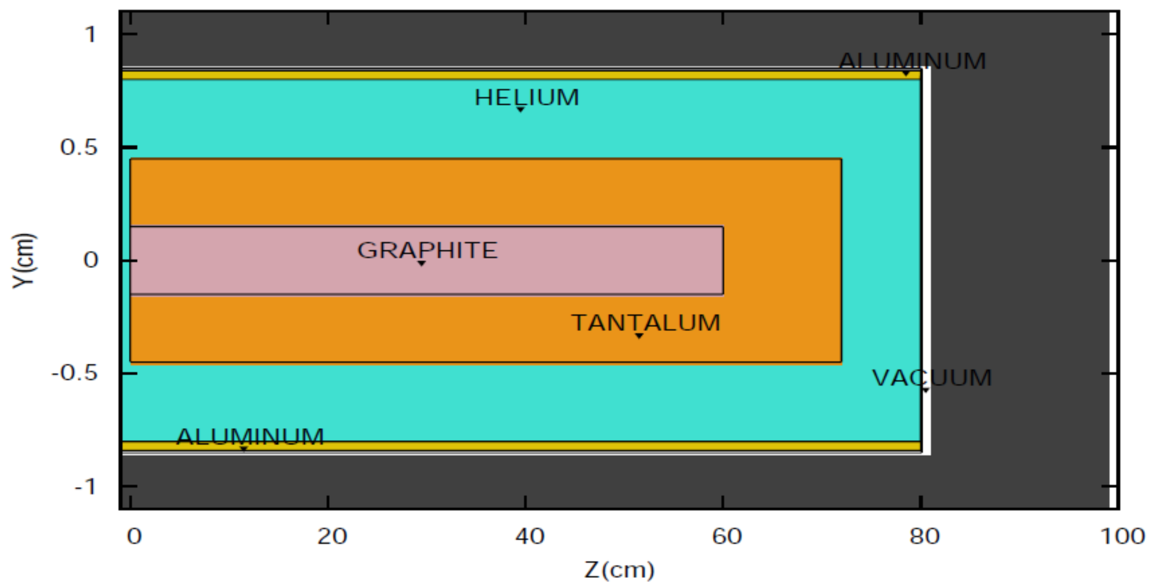
HYBRID GRAPHITE-TANTALUM TARGET Y-Z
