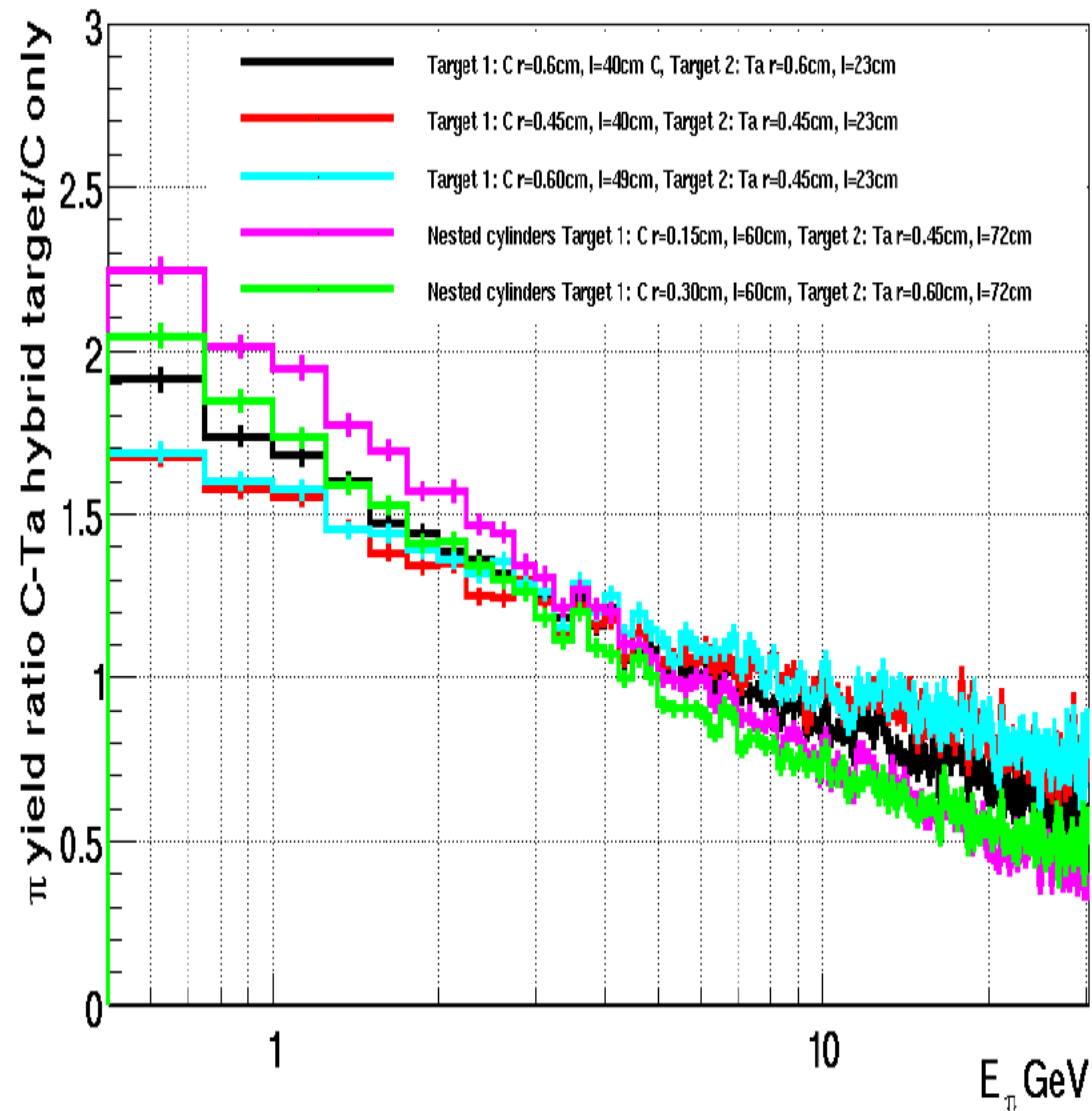
Pion yields from a hybrid C-Ta target at 120 GeV
